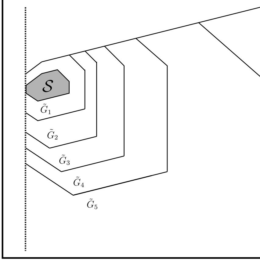
FIGURE 7. The sets \mathcal{S} \subseteq \tilde{G}_1 \subseteq \tilde{G}_2 \subseteq \cdots \subset G_\omega .
